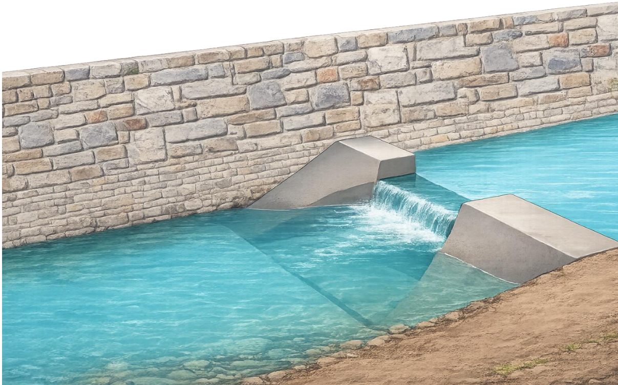
Figure 2: A slot cut into a weir without further easement measures. If the slot were small enough to be drowned out simply by restricting its cross-sectional area, the resulting water velocity would be too great for effective upstream passage.
